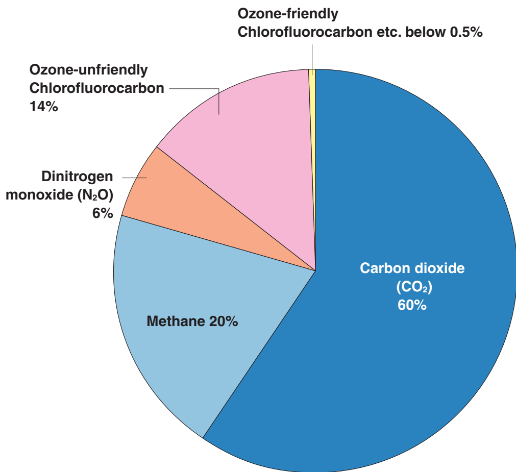
Direct contribution to global warming of GHGs emitted by human activities after the Industrial Revolution
