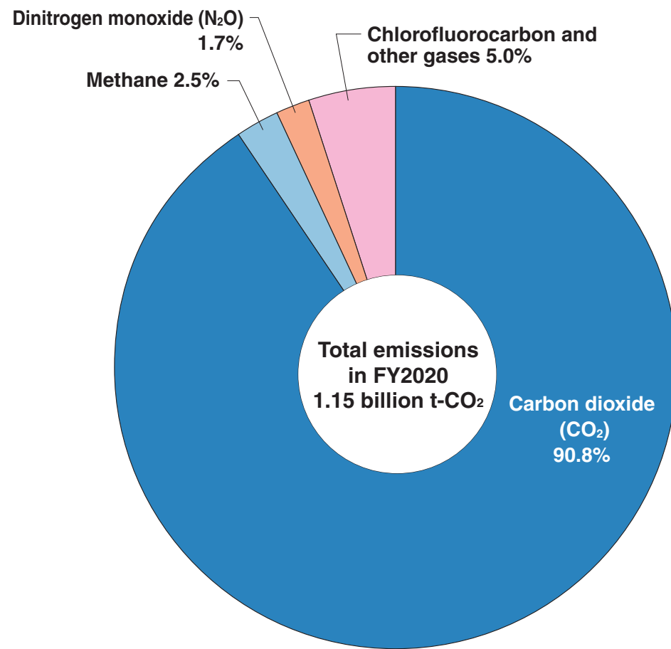
Direct contribution to global warming of GHGs emitted by Japan (for the single year of fiscal 2020)
